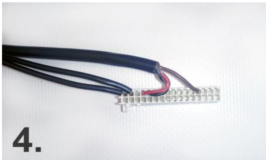
On 32 pin terminal connect bigger silver pins on position 7 and 8.
